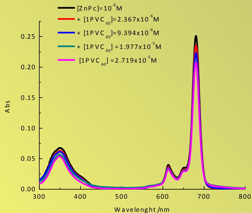
Absorption spectra in chlorobenzene of ZnPc ( 1.0 \times 10^{-6} M ) with variable concentrations of C_{60} -PPV1-pyr ( 0 - 2.7 \times 10^{-5} M )
