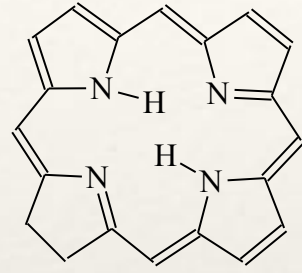
chlorin (2,3 dihydroporphyrin)
