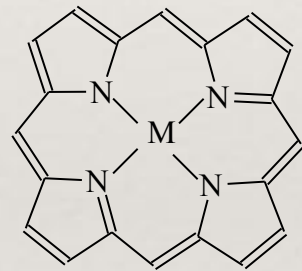
metalloporphyrin complex
