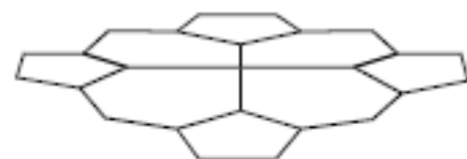
sad ( B_{2u} ), 65\text{ cm}^{-1}
