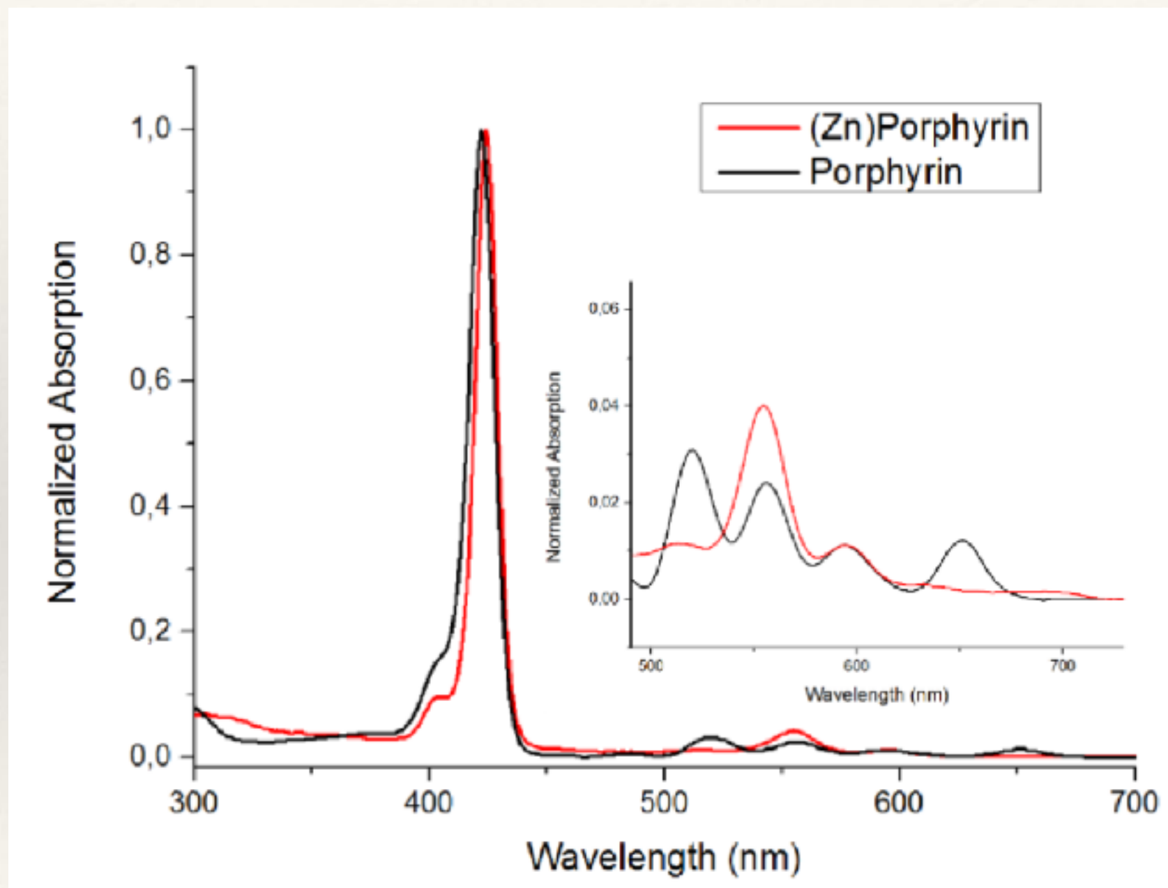
The UV-Vis absorption spectra of a free base porphyrin (black line) and a zinc metallated porphyrin (red line).
